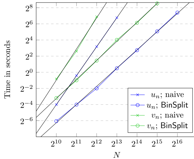
Figure 3: Timings for computing the N -th term of integer q -holonomic sequences u_n = [n]_3! and v_n = \sum_{i=1}^{n-1} 2^{i^2} for various values of N with Algorithm 5 (BinSplit) and naively.
